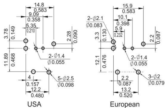
安装尺寸图 (底视图) Mounting (Bottom view)
