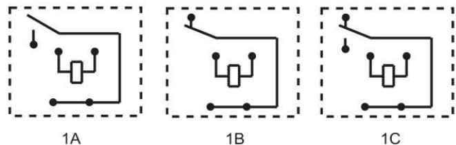
接线图 (底视图) Wiring diagram (Bottom view)
