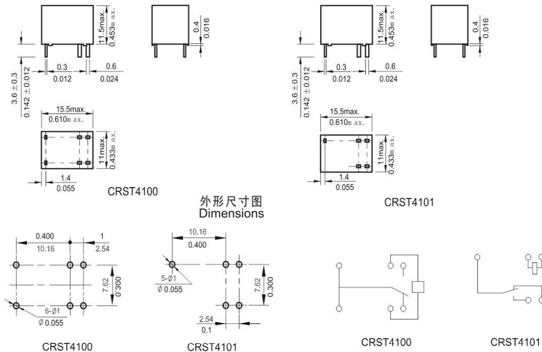
安装尺寸图 (底视图) Mounting (Bottom view)
