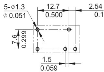
安装尺寸图 (底视图) Mounting (Bottom view)
