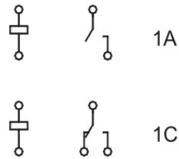
接线图 (底视图) Wiring diagram (Bottom view)
