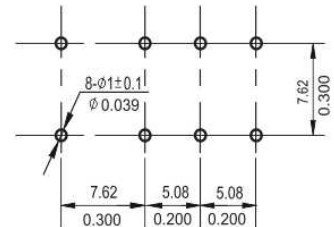
安装尺寸图 (底视图) Mounting (Bottom view)
