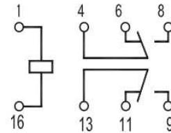
接线图 (底视图) Wiring diagram (Bottom view)
